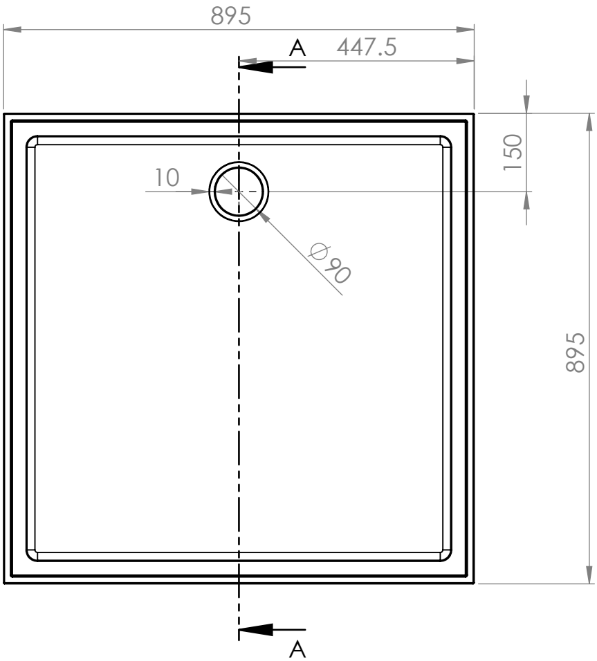
TOP VIEW
