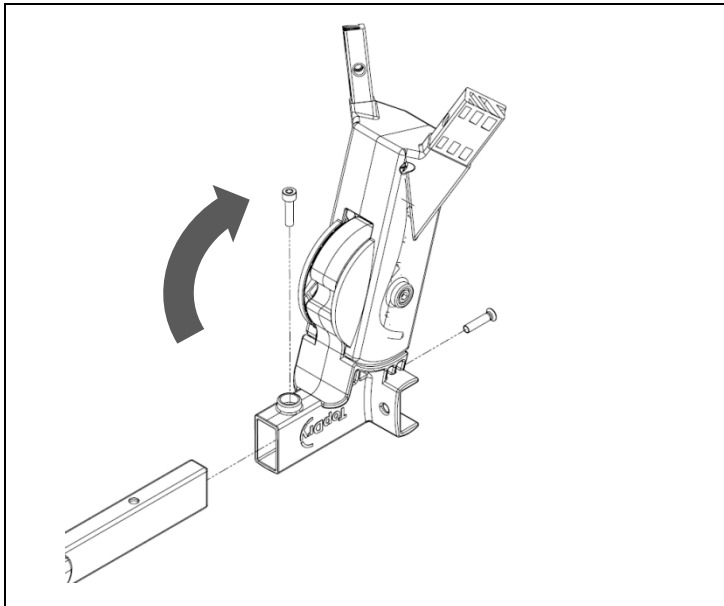
Step 3 – Rotate the Pivot to the open position and secure to the Spreader with screws (14 and 15).
