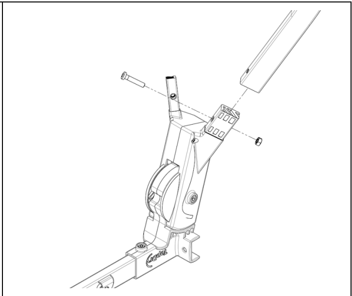
Step 4 –Fit the Legs and secure with screws (13) and nuts (9). Repeat for all legs.
