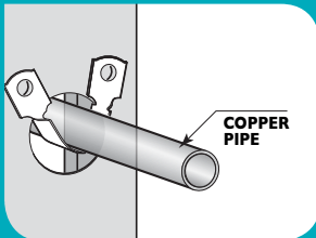
Side Saddle Clips in steel frame application
