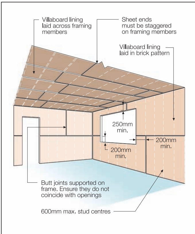
FIGURE 2 SHEET LAYOUT
