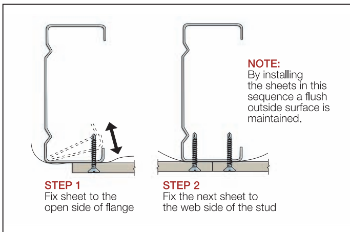
FIGURE 7 SCREW FASTENING
