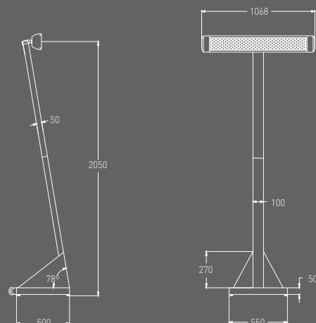
Note: Connection to power source is at bottom of stand, not shown in image. Measurements are in mm
