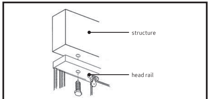
Diagram B. Align headrail under structure & mark where hole positions need to be located.
