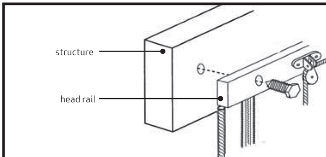
Diagram A. Align headrail onto face of structure & mark where hole positions need to be located.
