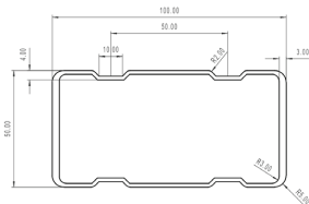
100 x 50 ALYSPAN Beam
