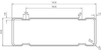
150 x 50 ALYSPAN Beam
