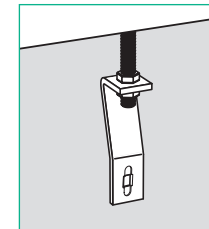
Fit All Thread Bracket to threaded rod with nuts provided.
