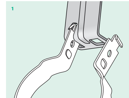
Step 1 – Engage clip to bracket through keyhole slot.
