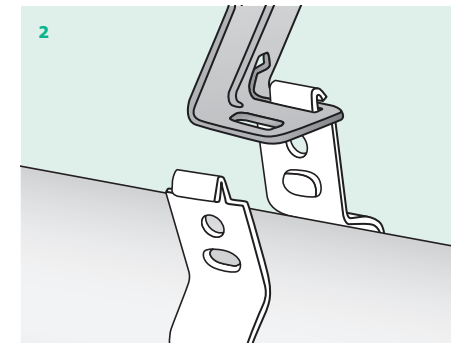
Step 2 – Install pipe as required. Pipes can be pre-hung.
