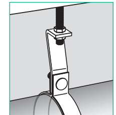
Fit bolted clip and pipe as required and adjust to pipe fall.
