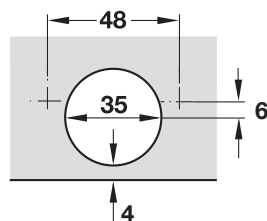
Salice Hinge Drilling Pattern
