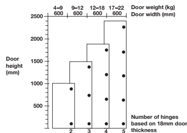
Salice Hinge Drilling Pattern
