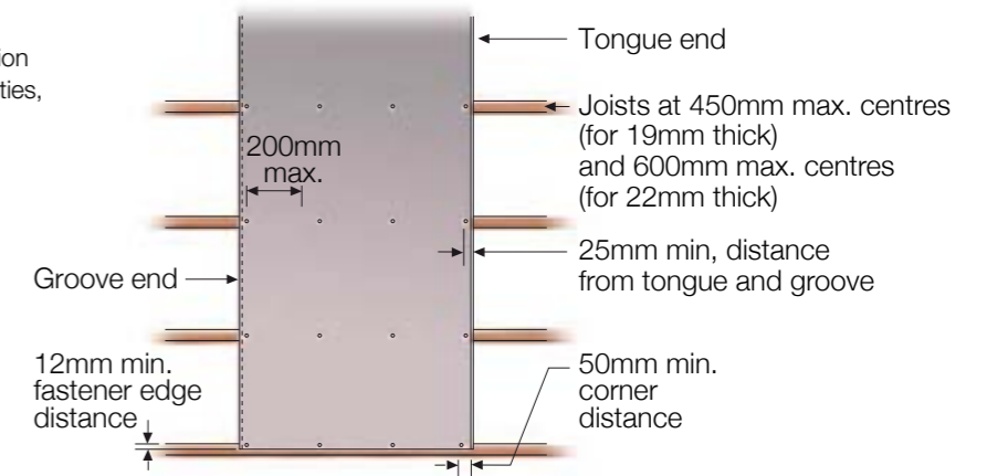
Scyon™ Secura™ Interior fastener layout
