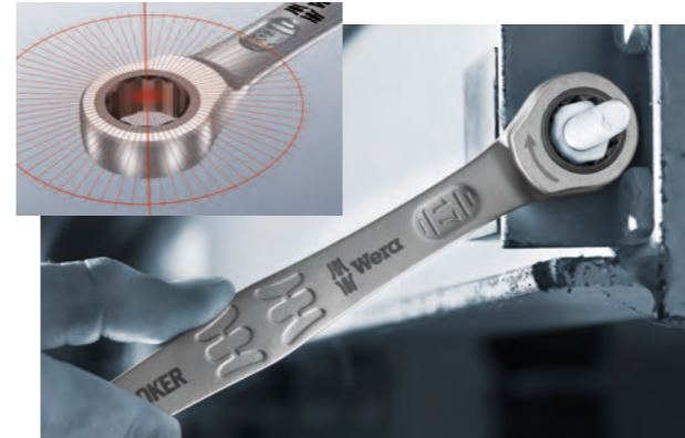
Fine tooth mechanism with 80 teeth.
