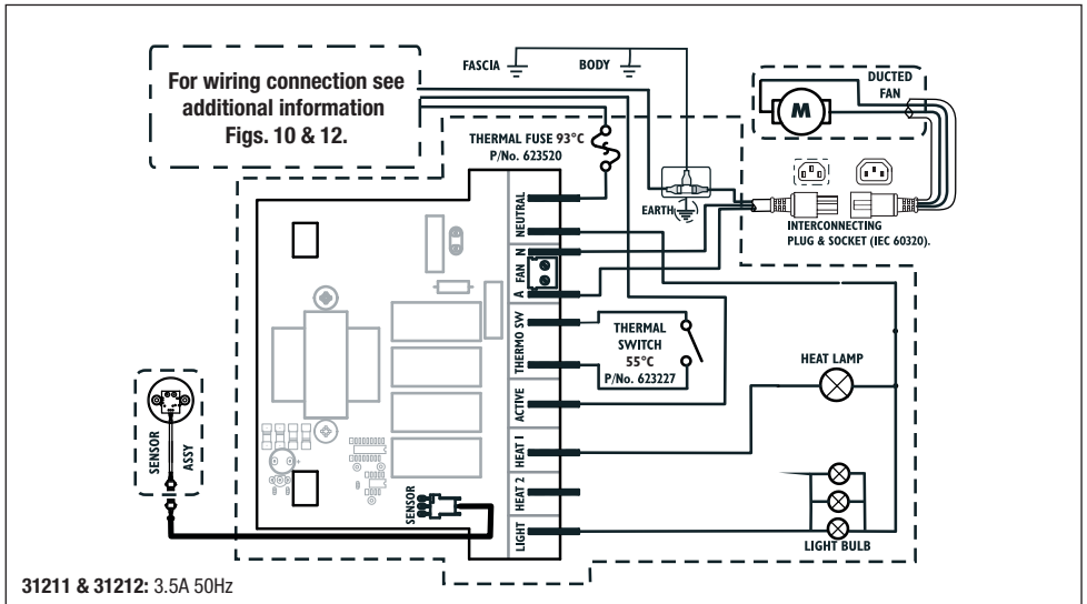
Fig. 5: Wiring diagram for models 31211 and 31212.
