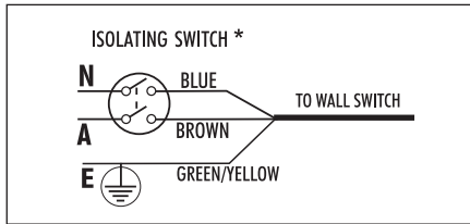
Fig. 10: Hardwired
