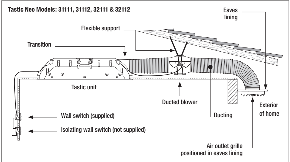
Fig. 3: Layout of Tastic Neo Single and Dual.
