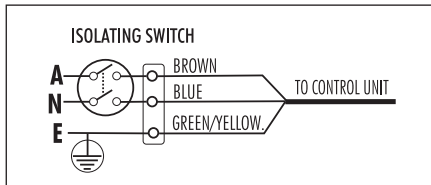
Fig. 11: Smart Switch
