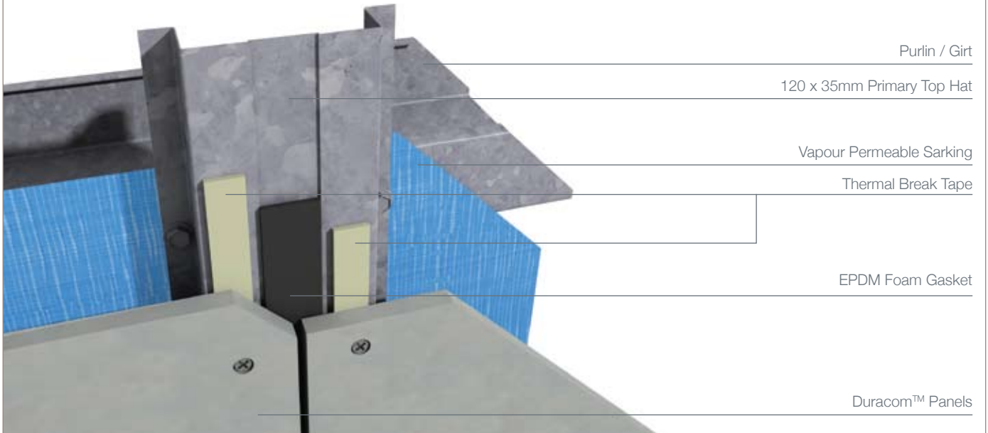
THERMAL BREAK DETAIL
