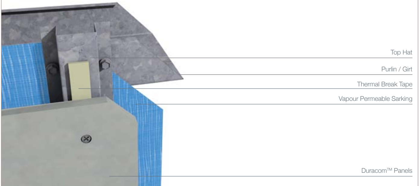
THERMAL BREAK DETAIL
