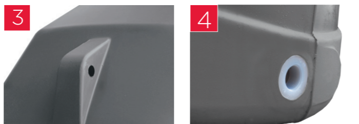
Moulded lugs for easy lifting and tie-down points
