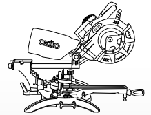
Compound Mitre Saw
