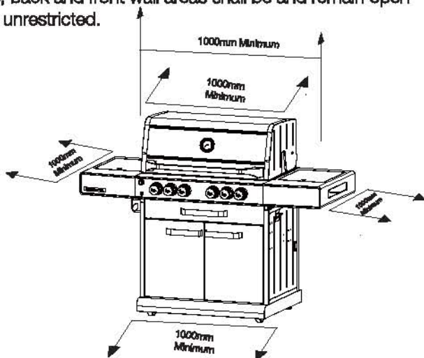
Minimum Distances from Combustible Material
