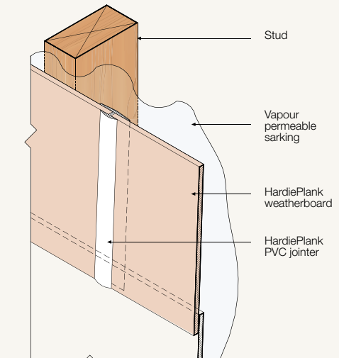
Figure 8 PVC jointer
