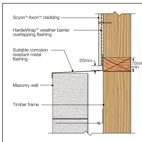
FIGURE 26 HORIZONTAL JUNCTION 2
