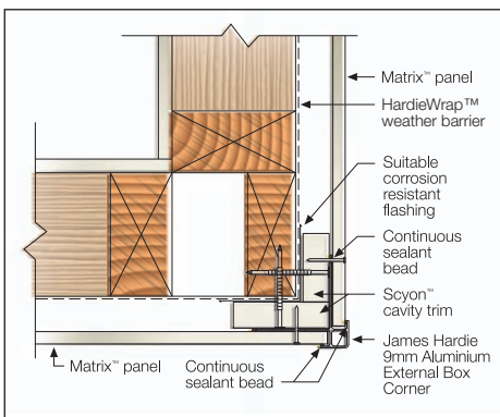
FIGURE 26 SCYON MATRIX EXTERNAL BOX CORNER DETAIL
