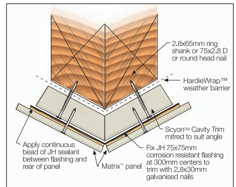
FIGURE 32 ANGLED CORNER
