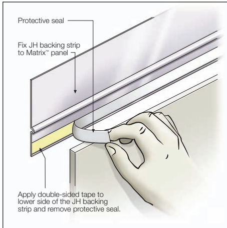
FIGURE 12 DOUBLE SIDED BACKING TAPE OPTION 2
