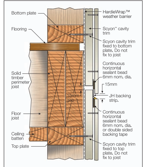
FIGURE 30 FLOOR LEVEL JUNCTION
