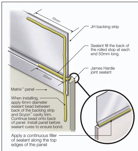
FIGURE 13 SEALING JH BACKING STRIP END DETAIL
