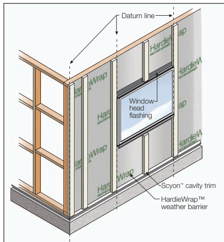
FIGURE 6 PANEL LAYOUT
