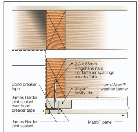
FIGURE 31 ABUTMENT DETAIL
