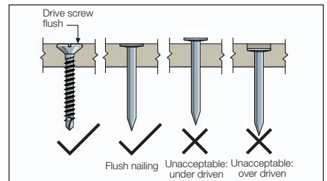
FIGURE 2 NAIL FASTENER DEPTH
