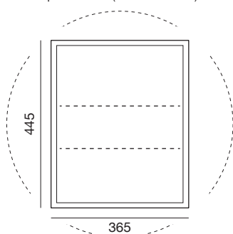
Front View Open Cabinet (mirror indicated)
