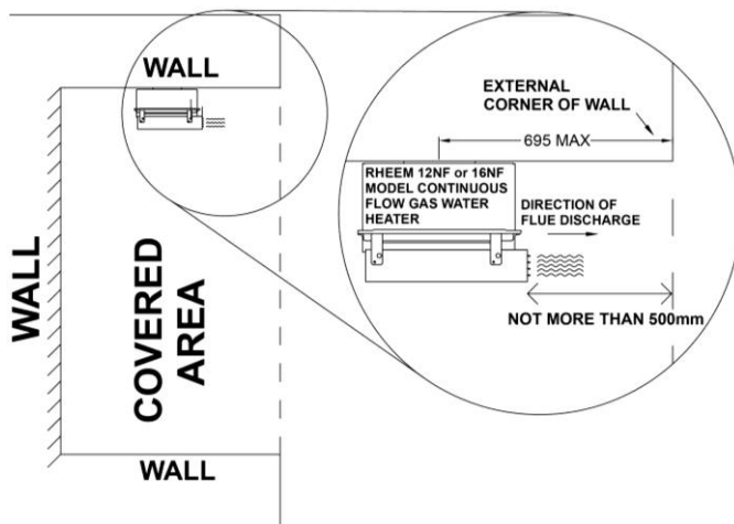
12NF or 16NF model with a Flue Terminal Diverter installed in compliance with AS/NZS 5601.1
