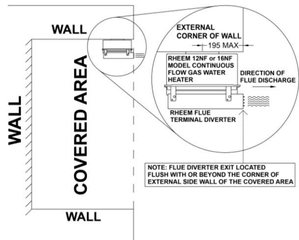
12NF or 16NF model with a Flue Terminal Diverter installed in compliance with AS 5601 and AS/NZS 5601.1
