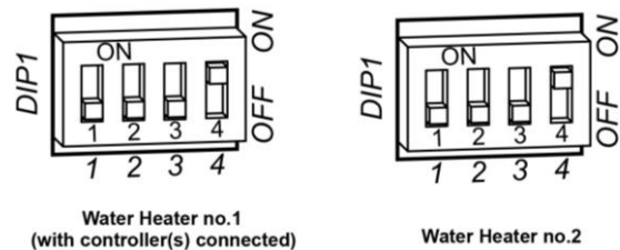
dip switch settings with temperature controller connected
